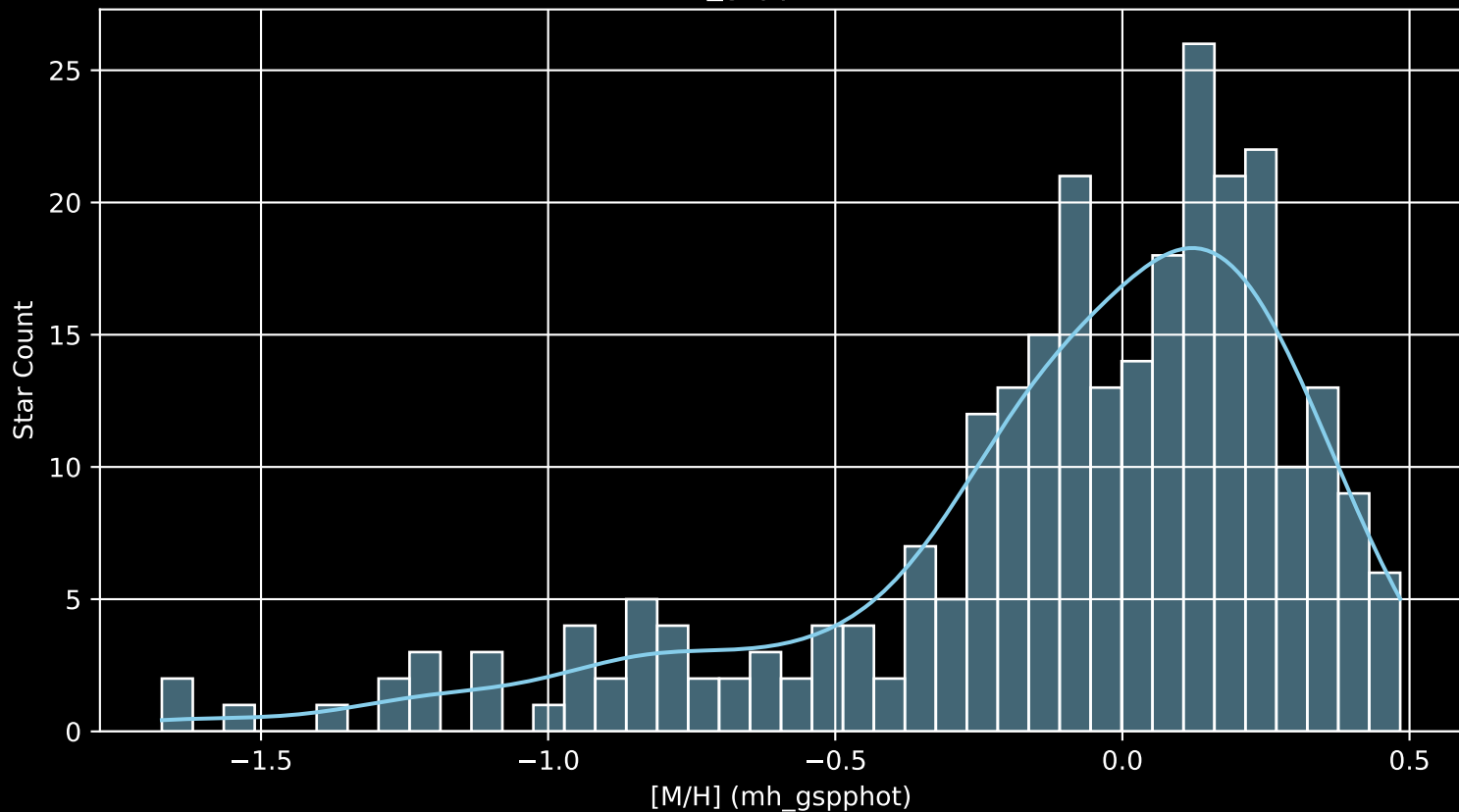
APOGEE DR17 Field: [010-04 [M/H] (mh_gspphot) (n= 272)
