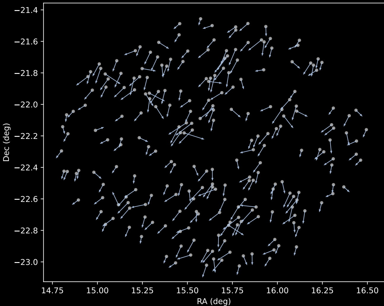
APOGEE DR17 Cluster 1 Proper Motion Vectors (n=233)
