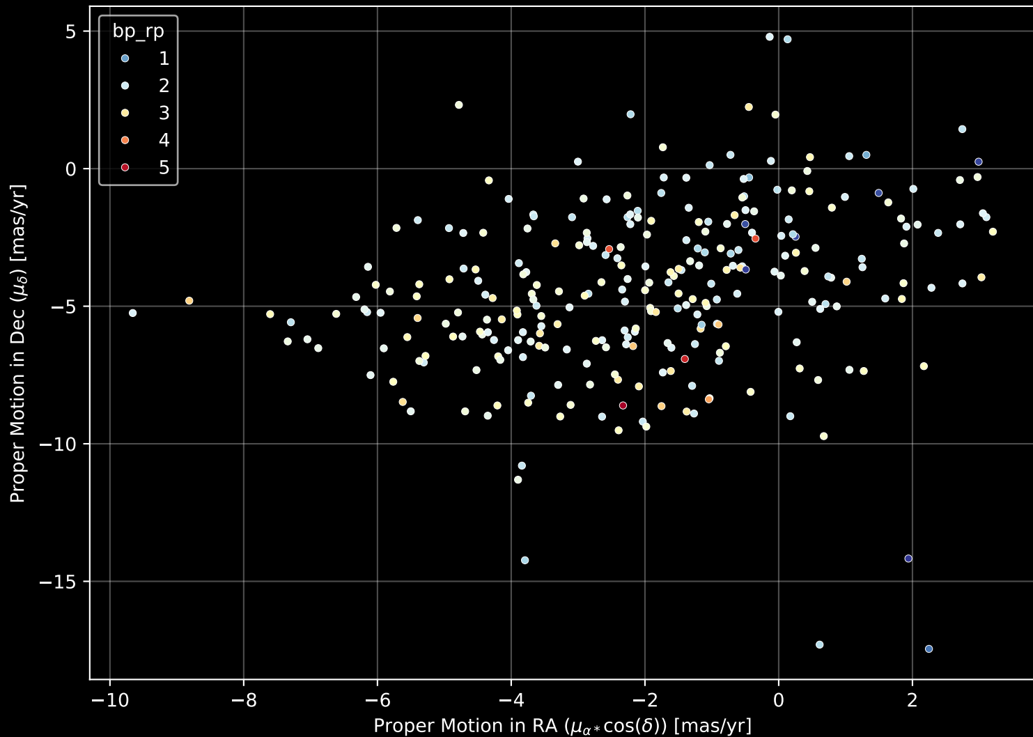
APOGEE DR17 Field: [010-04] Proper Motion Diagram (n= 282)
