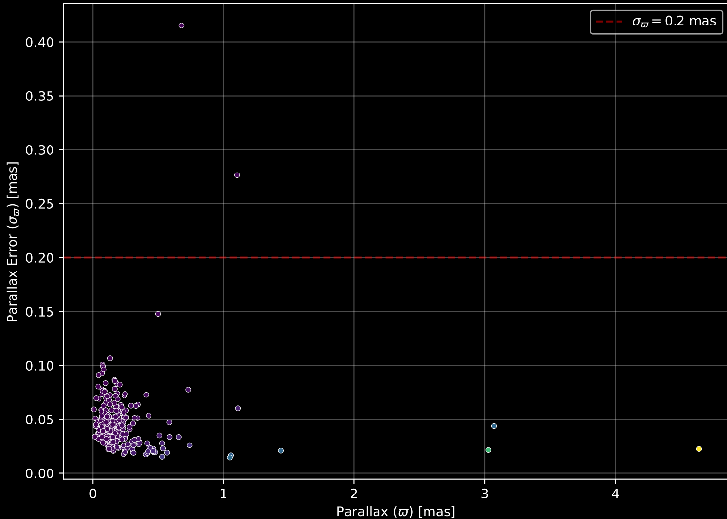
APOGEE DR17 Field: [010-04] Parallax Quality (n= 282)
