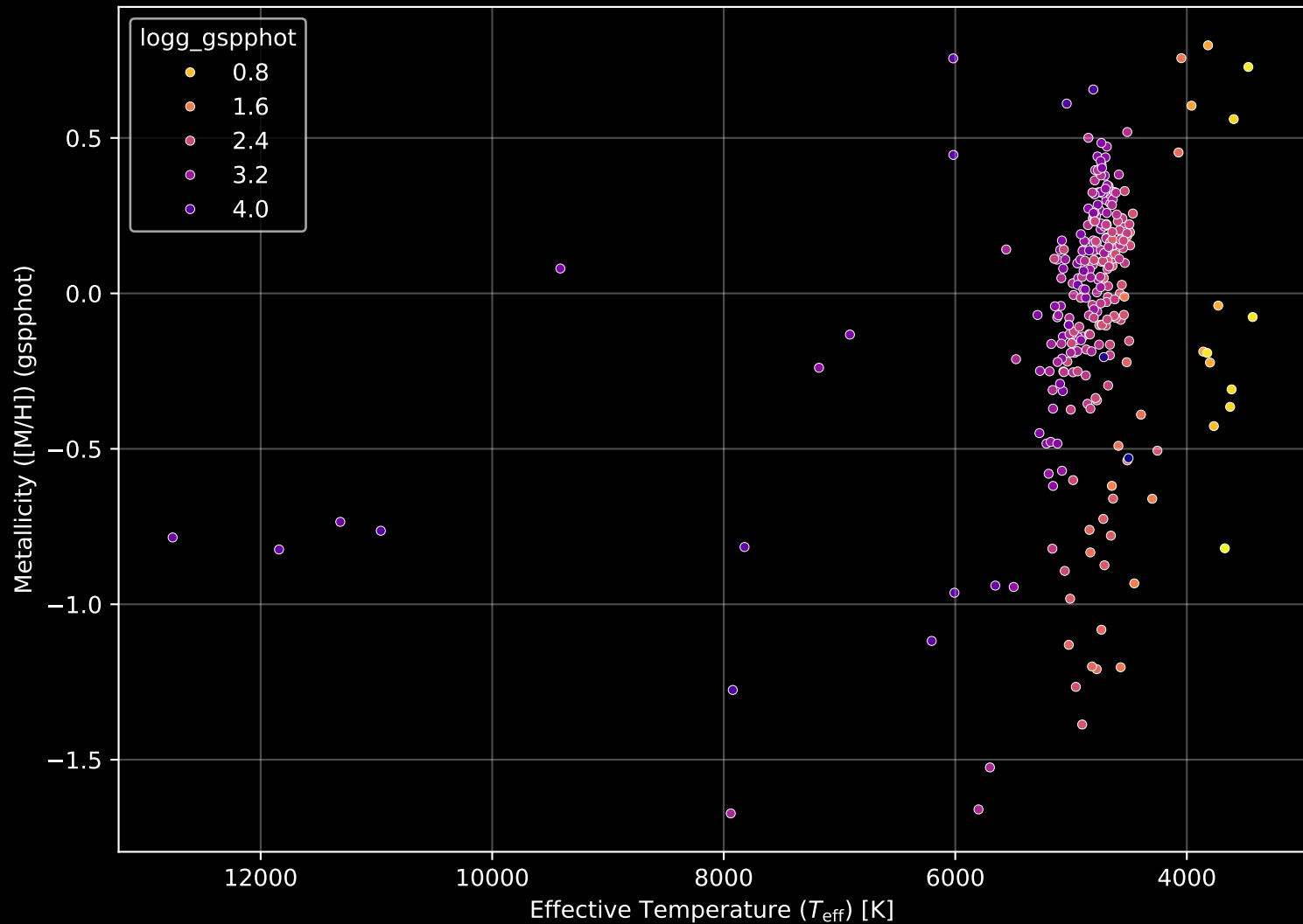
APOGEE DR17 Field: [010-04] Stellar Population Parameters (n= 282)
