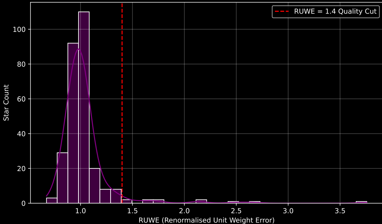
GAPOGEE DR17 Field [010-04] RUWE Distribution (n= 281)
